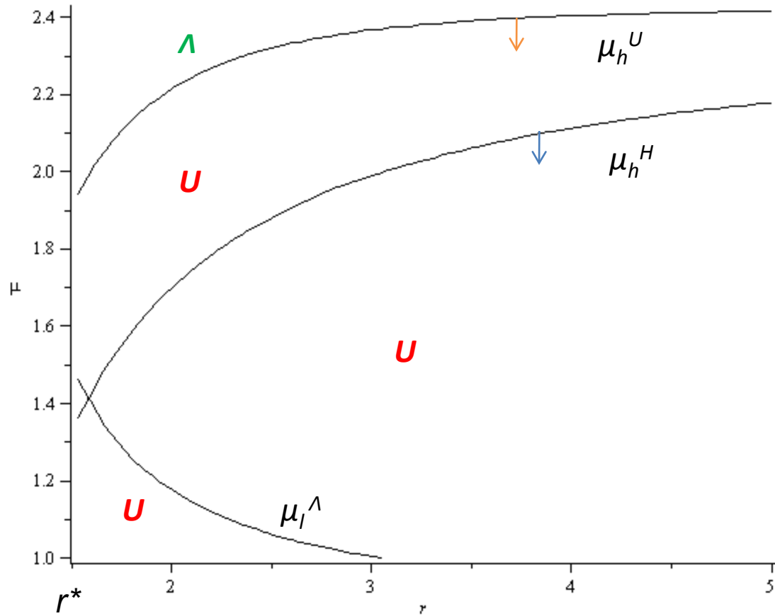
Fig 3: Equilibrium market structure under (P, P)
